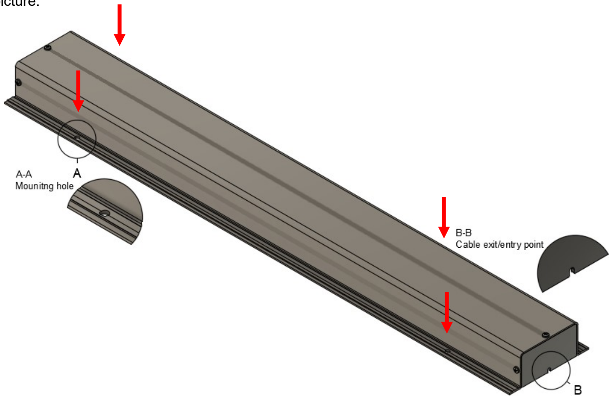
Figure 1: Installation possibilities of the OPC-02 protection cover.
