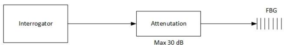
Figure 1: Max. allowed attenuation within optical line (bidirectional)
