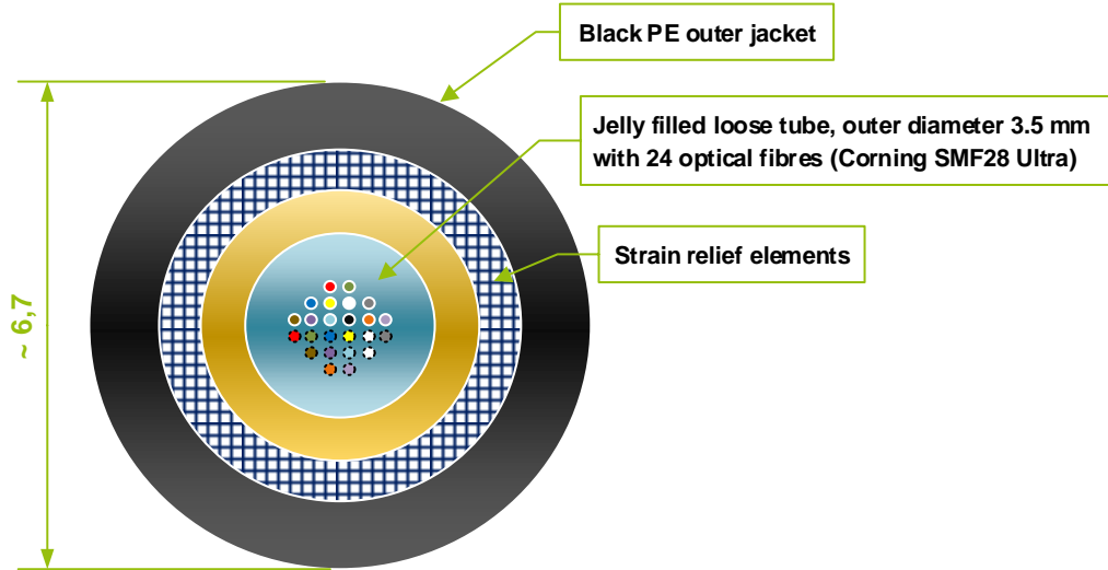
Example of 24 fibers cable
